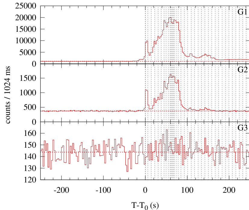
Konus-WIND S2 SOL2012-05-10T04:15 (M5.7) T 0 = 15321.348 s UT (04:15:21.348)
