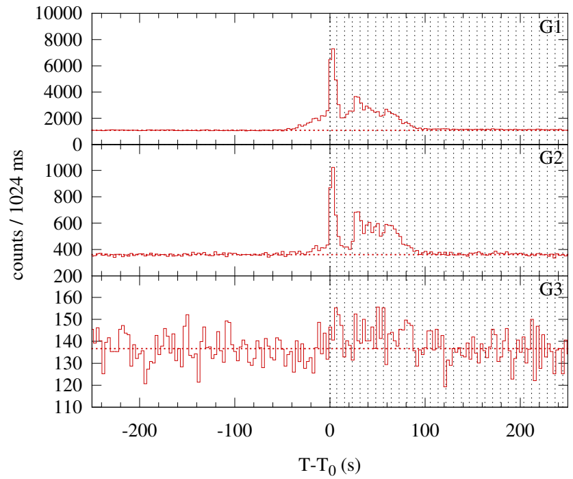
Konus-WIND S2 SOL2012-06-09T11:30 (M1.9) T 0 = 41453.76 s UT (11:30:53.76)
