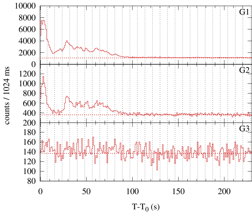
Konus-WIND S2 SOL2012-06-09T11:30 (M1.9) T 0 = 41453.76 s UT (11:30:53.76)
