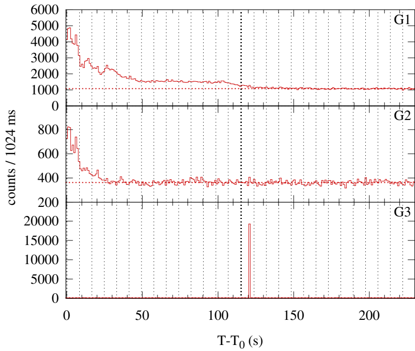
Konus-WIND S2 SOL2012-07-05T10:46 (M1.8) T 0 = 38798.179 s UT (10:46:38.179)
