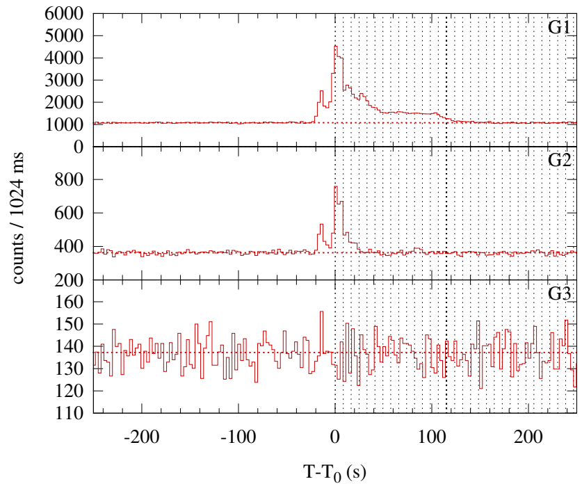
Konus-WIND S2 SOL2012-07-05T10:46 (M1.8) T 0 = 38798.179 s UT (10:46:38.179)
