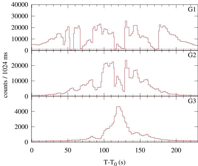
Konus-WIND S2 SOL2012-07-06T23:04 (X1.1) T_0 = 83070.651 s UT (23:04:30.651)
