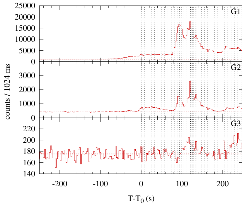
Konus-WIND S2 SOL2012-07-08T16:24 (M6.9) T 0 = 59099.98 s UT (16:24:59.98)
