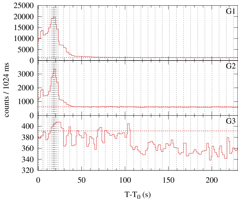
Konus-WIND S2 SOL2012-07-09T23:06 (M1.1) T_0 = 83189.395 s UT (23:06:29.395)
