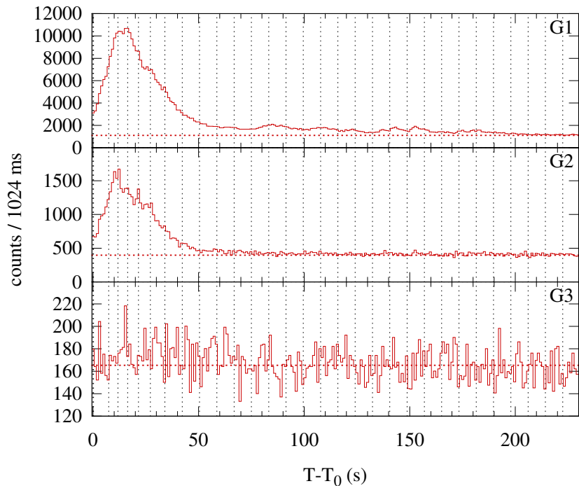
Konus-WIND S2 SOL2012-08-06T04:35 (M1.6) T_0 = 16540.760 s UT (04:35:40.760)
