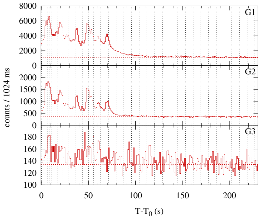
Konus-WIND S2 SOL2012-08-18T03:21 (M1.8) T_0 = 12084.363 s UT (03:21:24.363)
