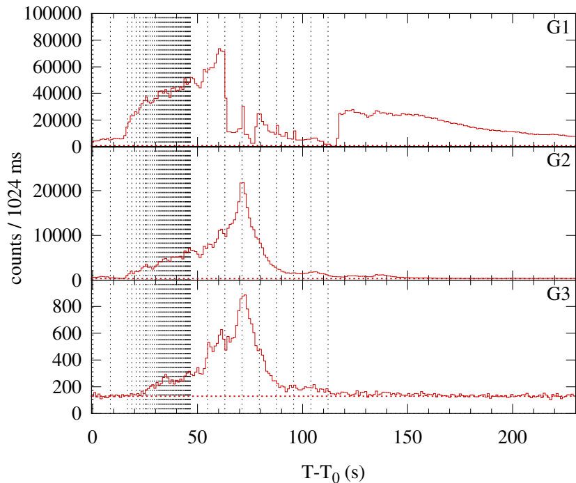
Konus-WIND S2 SOL2012-10-23T03:14 (X1.8) T_0 = 11680.760 s UT (03:14:40.760)
