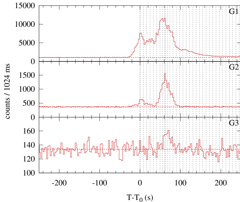
Konus-WIND S2 SOL2012-11-13T02:01 (M6.0) T 0 = 7295.536 s UT (02:01:35.536)
