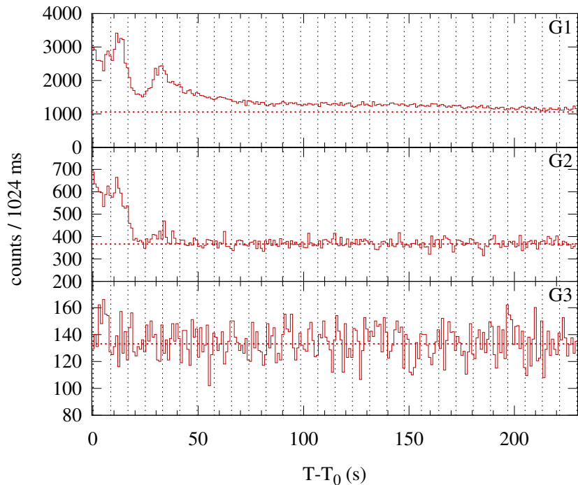
Konus-WIND S2 SOL2012-11-13T05:47 (M2.5) T_0 = 20834.938 s UT (05:47:14.938)
