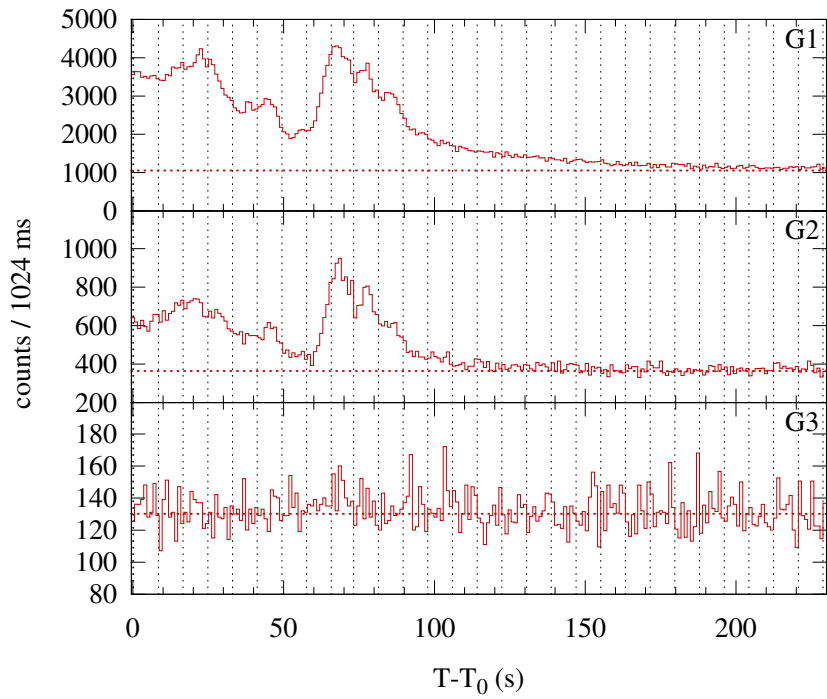
Konus-WIND S2 SOL2012-11-13T20:52 (M2.8) T_0 = 75150.848 s UT (20:52:30.848)
