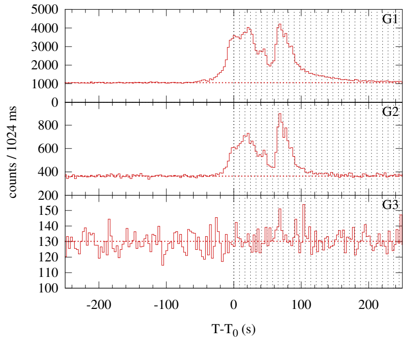
Konus-WIND S2 SOL2012-11-13T20:52 (M2.8) T_0 = 75150.848 s UT (20:52:30.848)
