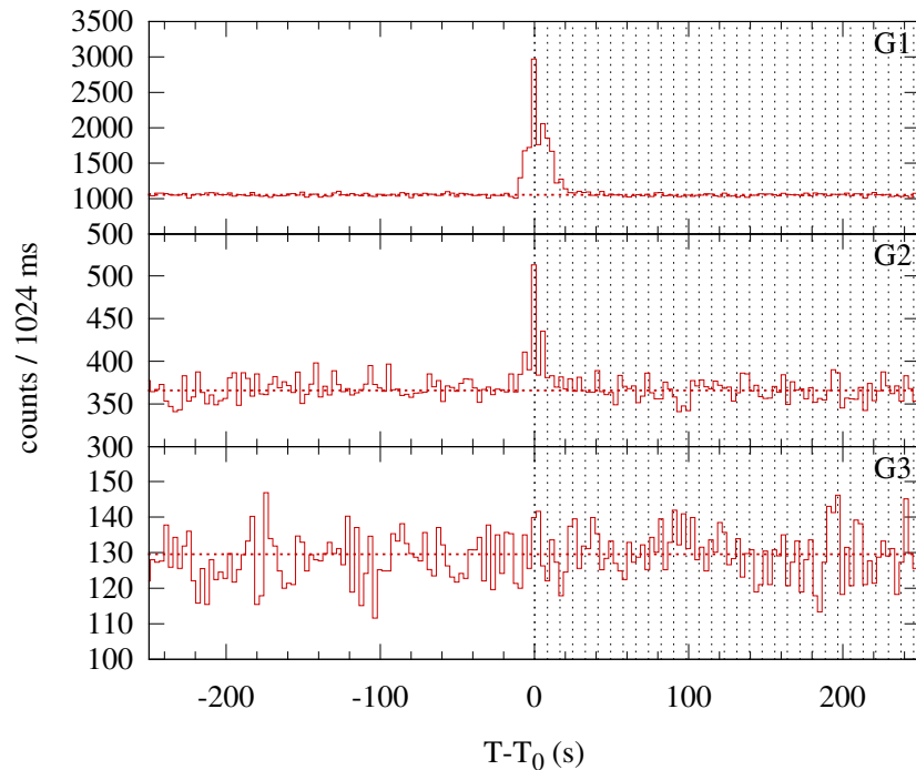
Konus-WIND S2 SOL2012-11-23T19:29 (C2.5) T 0 = 70169.819 s UT (19:29:29.819)
