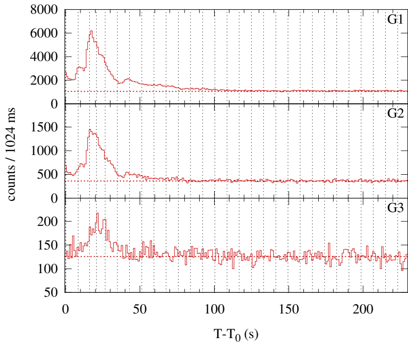
Konus-WIND S2 SOL2012-11-27T15:55 (M1.6) T_0 = 57341.118 s UT (15:55:41.118)
