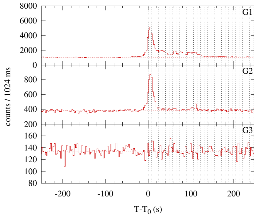
Konus-WIND S2 SOL2013-01-13T00:48 (M1.0) T 0 = 2901.937 s UT (00:48:21.937)
