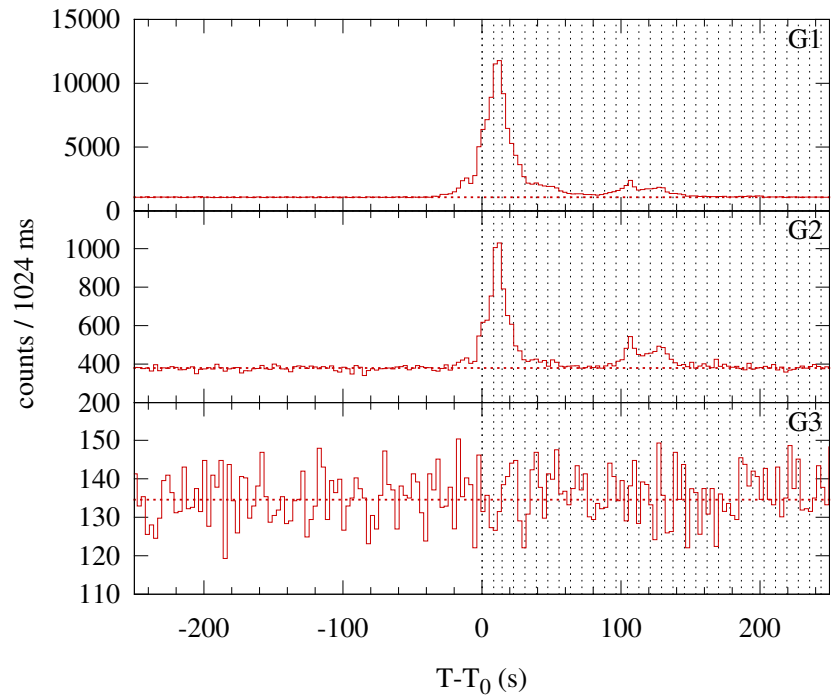
Konus-WIND S2 SOL2013-01-13T08:36 (M1.7) T 0 = 30983.185 s UT (08:36:23.185)
