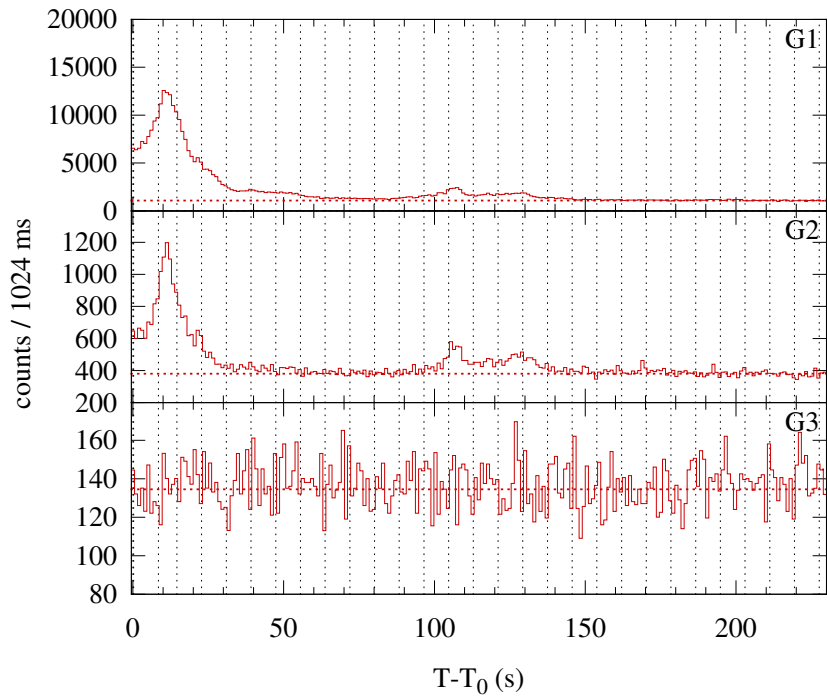
Konus-WIND S2 SOL2013-01-13T08:36 (M1.7) T 0 = 30983.185 s UT (08:36:23.185)
