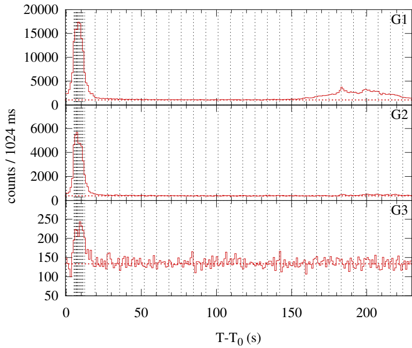
Konus-WIND S2 SOL2013-02-17T15:47 (M1.9) T 0 = 56827.781 s UT (15:47:07.781)
