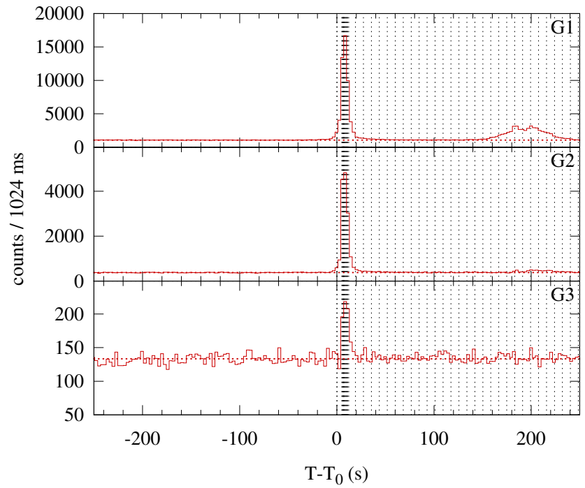
Konus-WIND S2 SOL2013-02-17T15:47 (M1.9) T 0 = 56827.781 s UT (15:47:07.781)
