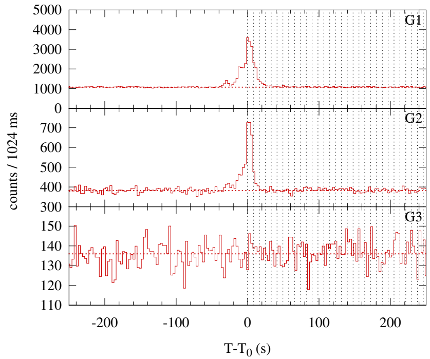
Konus-WIND S2 SOL2013-02-20T11:10 (C8.2) T 0 = 40257.236 s UT (11:10:57.236)
