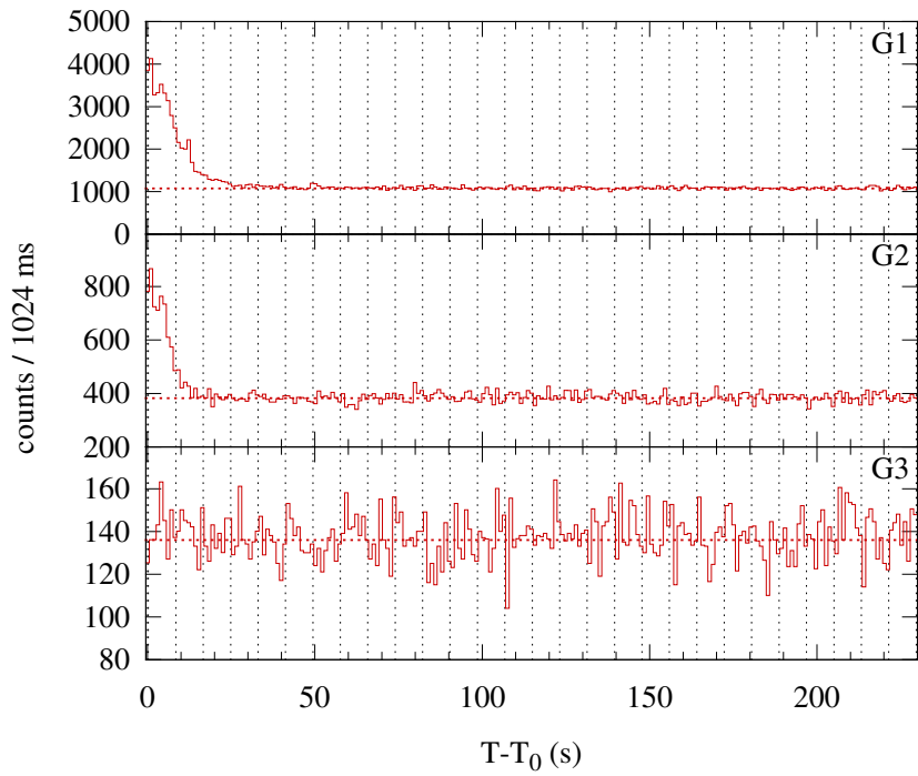
Konus-WIND S2 SOL2013-02-20T11:10 (C8.2) T 0 = 40257.236 s UT (11:10:57.236)
