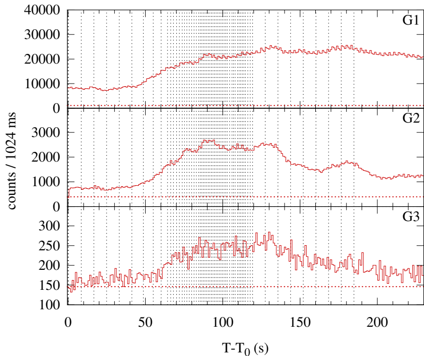
Konus-WIND S2 SOL2013-05-14T01:05 (X3.2) T_0 = 3920.916 s UT (01:05:20.916)
