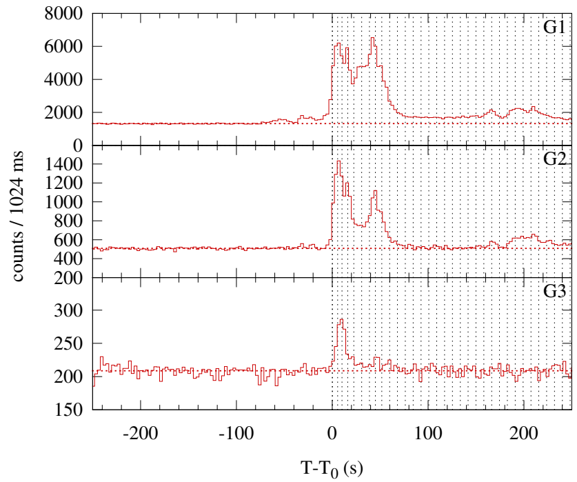
Konus-WIND S2 SOL2013-06-23T20:52 (M2.9) T_0 = 75164.163 s UT (20:52:44.163)
