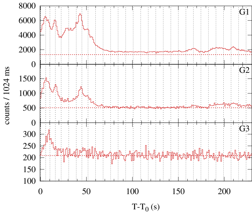
Konus-WIND S2 SOL2013-06-23T20:52 (M2.9) T_0 = 75164.163 s UT (20:52:44.163)
