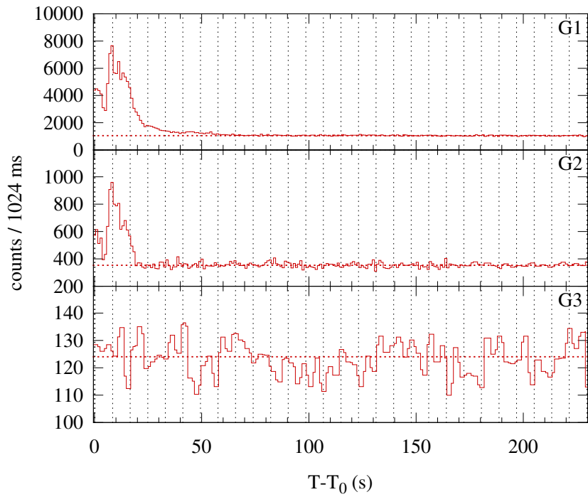
Konus-WIND S2 SOL2013-07-08T01:21 (C9.7) T_0 = 4913.240 s UT (01:21:53.240)
