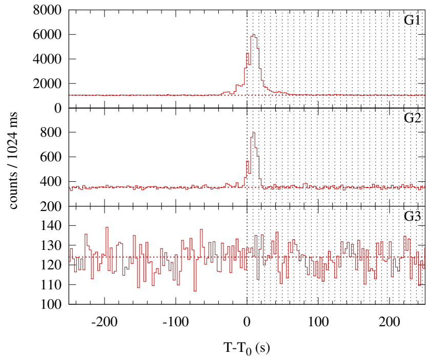
Konus-WIND S2 SOL2013-07-08T01:21 (C9.7) T_0 = 4913.240 s UT (01:21:53.240)
