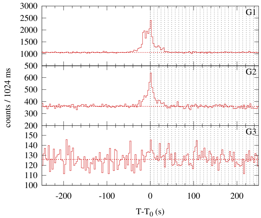
Konus-WIND S2 SOL2013-08-19T09:13 (C2.2) T_0 = 33209.112 s UT (09:13:29.112)
