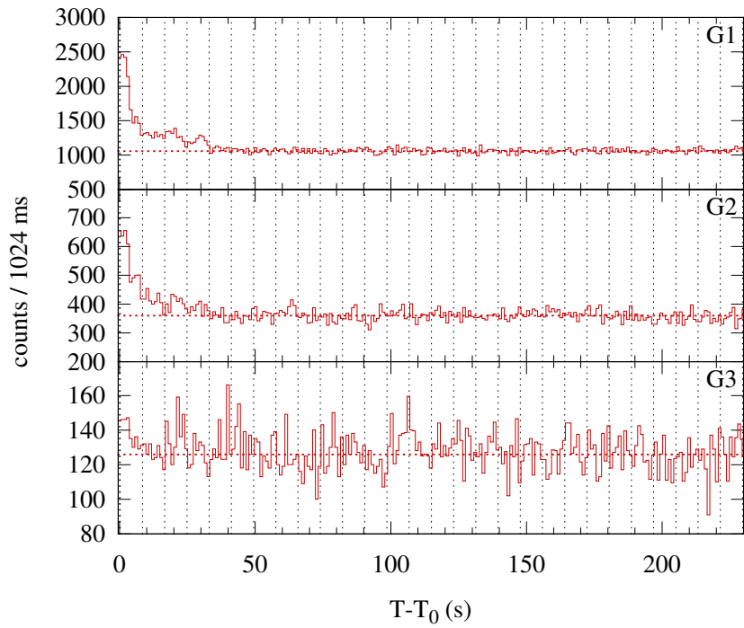
Konus-WIND S2 SOL2013-08-19T09:13 (C2.2) T_0 = 33209.112 s UT (09:13:29.112)
