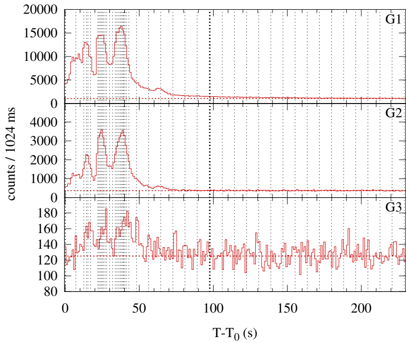
Konus-WIND S2 SOL2013-10-22T21:18 (M4.2) T_0 = 76717.380 s UT (21:18:37.380)
