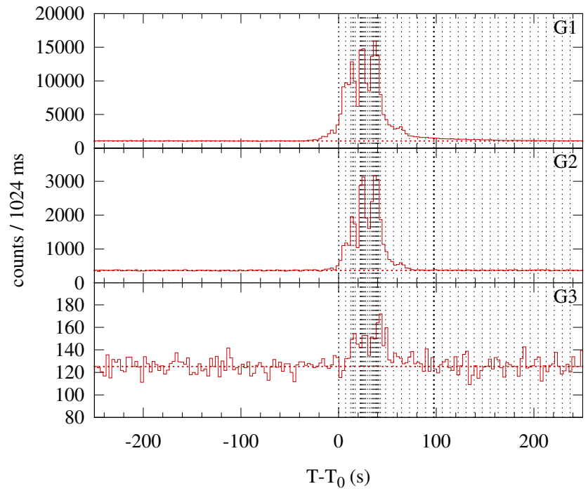
Konus-WIND S2 SOL2013-10-22T21:18 (M4.2) T_0 = 76717.380 s UT (21:18:37.380)
