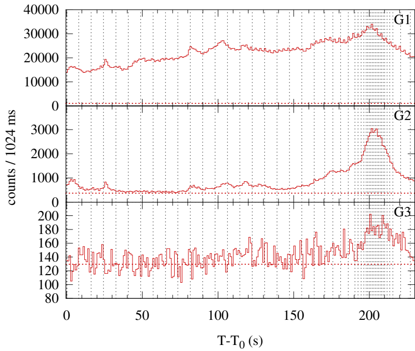
Konus-WIND S2 SOL2013-10-25T14:57 (X2.1) T_0 = 53830.821 s UT (14:57:10.821)
