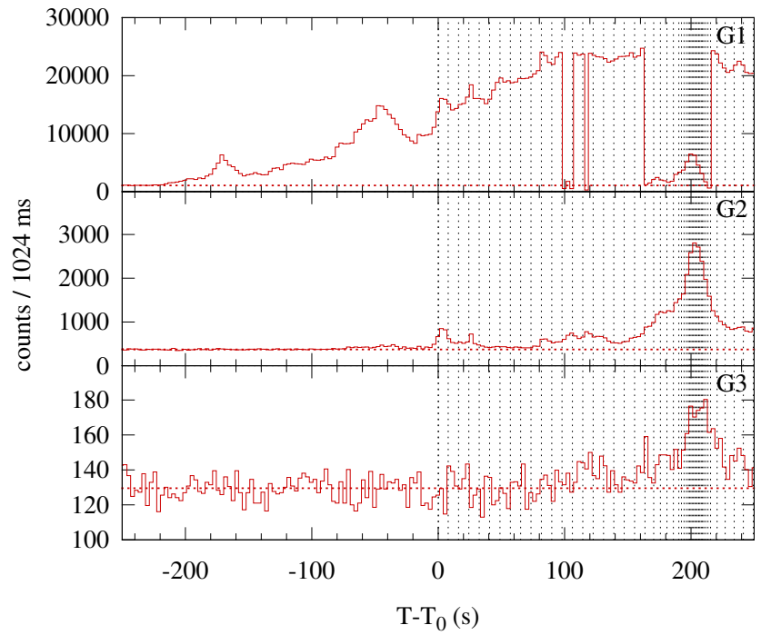
Konus-WIND S2 SOL2013-10-25T14:57 (X2.1) T_0 = 53830.821 s UT (14:57:10.821)
