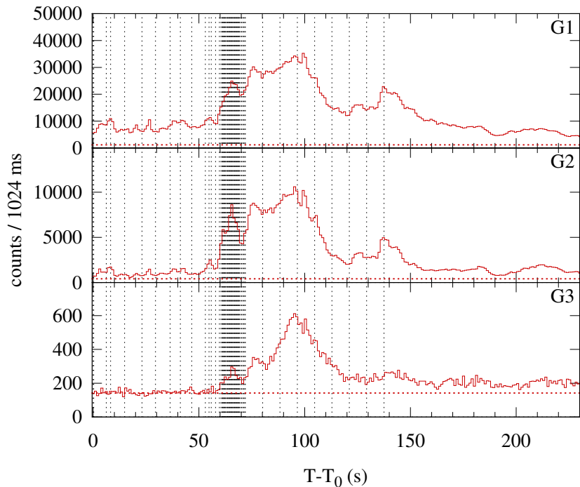
Konus-WIND S2 SOL2013-10-28T04:36 (M5.1) T_0 = 16600.634 s UT (04:36:40.634)
