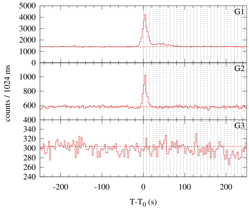
Konus-WIND S2 SOL2013-10-29T10:05 (C6.3) T_0 = 36314.370 s UT (10:05:14.370)
