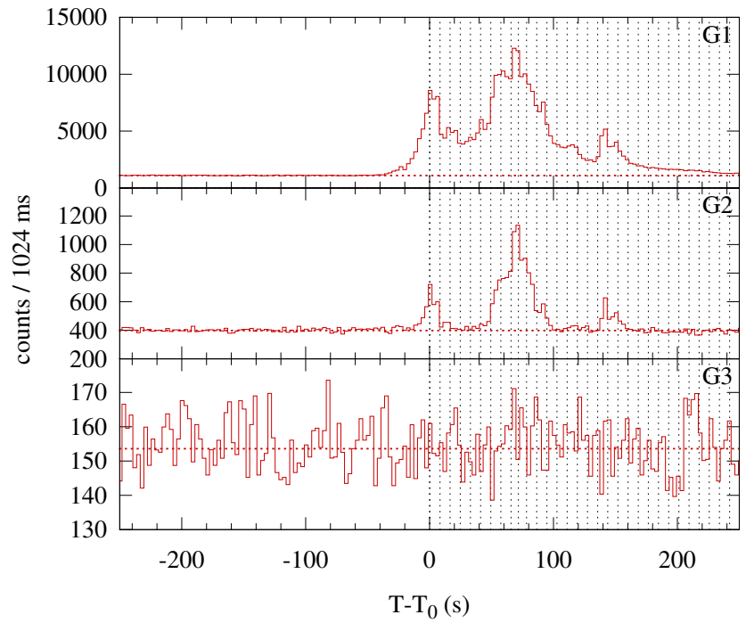
Konus-WIND S2 SOL2013-11-03T05:20 (M5.0) T_0 = 19221.807 s UT (05:20:21.807)
