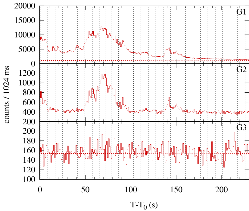
Konus-WIND S2 SOL2013-11-03T05:20 (M5.0) T_0 = 19221.807 s UT (05:20:21.807)
