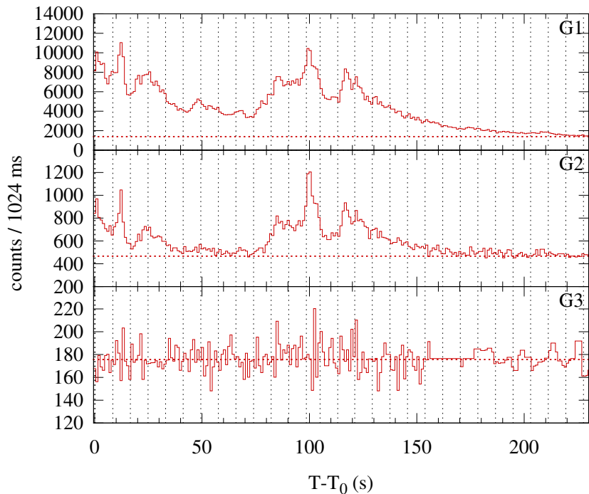
Konus-WIND S2 SOL2013-11-07T03:37 (M2.3) T 0 = 13069.89 s UT (03:37:49.89)
