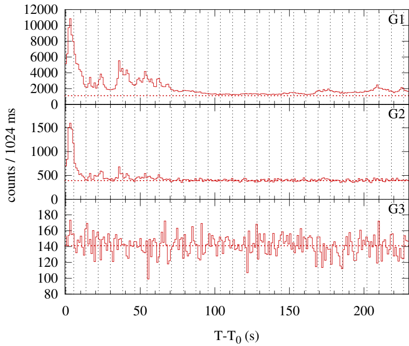
Konus-WIND S2 SOL2013-11-07T14:18 (M2.4) T 0 = 51493.612 s UT (14:18:13.612)
