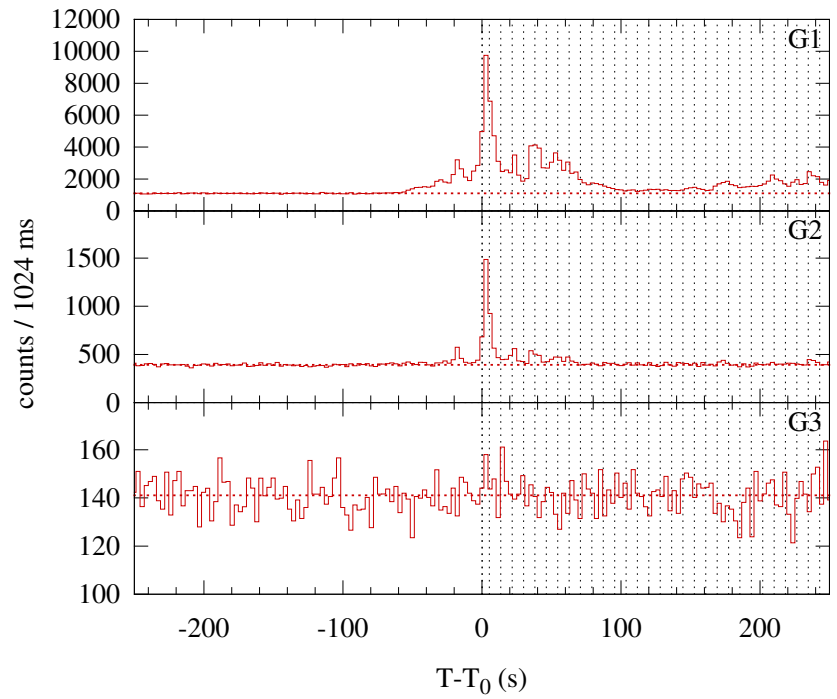
Konus-WIND S2 SOL2013-11-07T14:18 (M2.4) T 0 = 51493.612 s UT (14:18:13.612)
