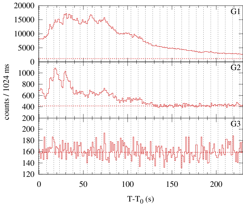
Konus-WIND S2 SOL2013-11-10T05:12 (X1.1) T_0 = 18722.285 s UT (05:12:02.285)
