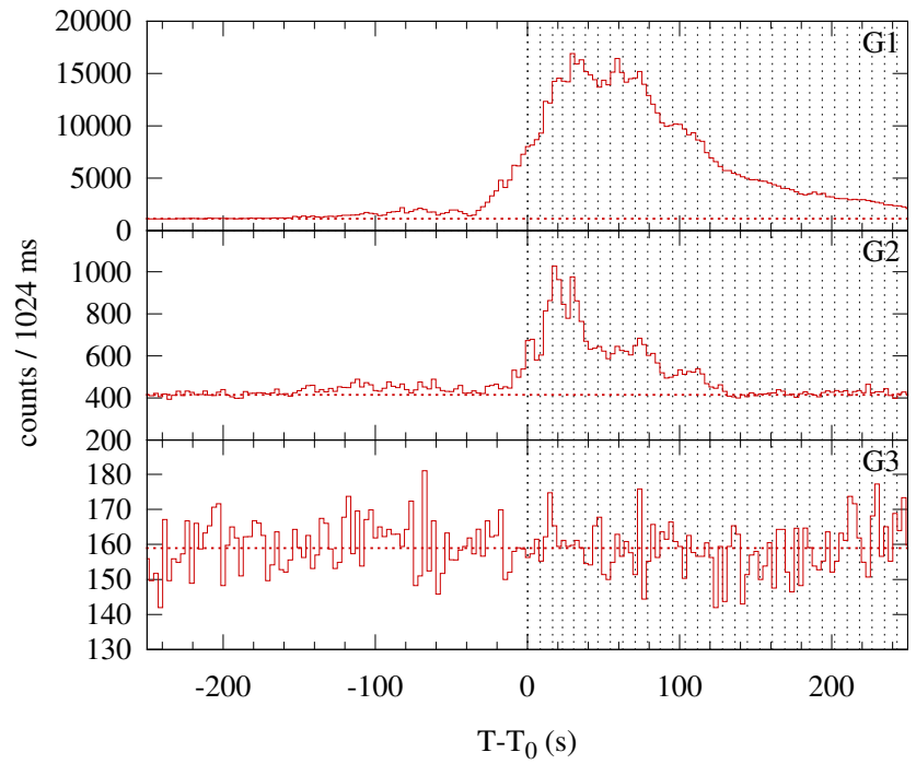
Konus-WIND S2 SOL2013-11-10T05:12 (X1.1) T_0 = 18722.285 s UT (05:12:02.285)
