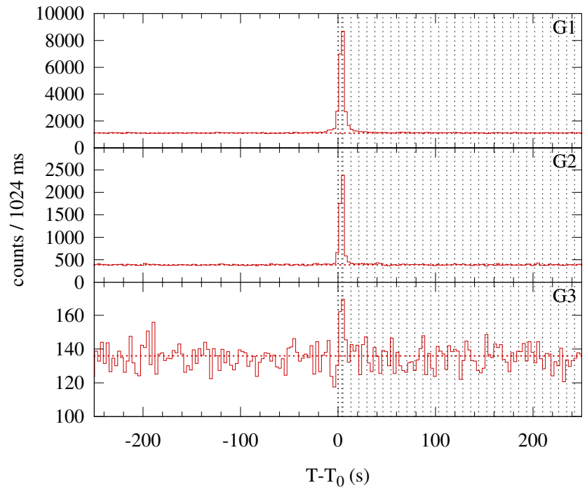
Konus-WIND S2 SOL2013-11-12T14:17 (C2.0) T 0 = 51423.243 s UT (14:17:03.243)
