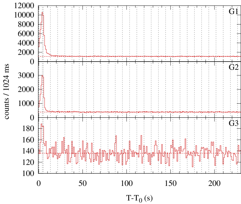
Konus-WIND S2 SOL2013-11-12T14:17 (C2.0) T 0 = 51423.243 s UT (14:17:03.243)
