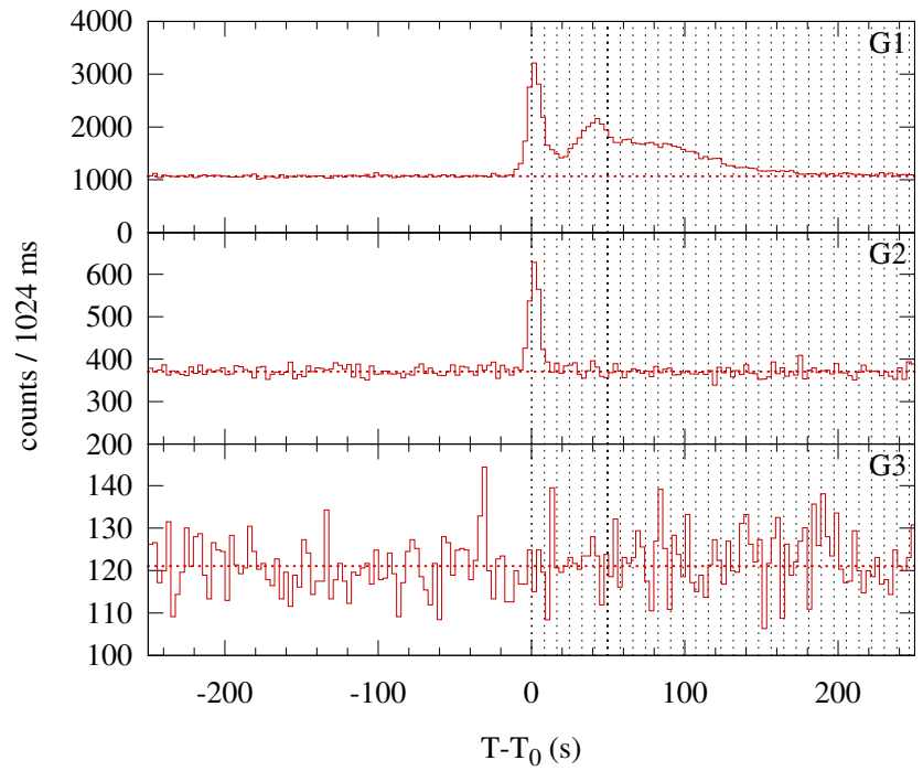
Konus-WIND S2 SOL2013-12-22T08:08 (M1.9) T_0 = 29331.393 s UT (08:08:51.393)
