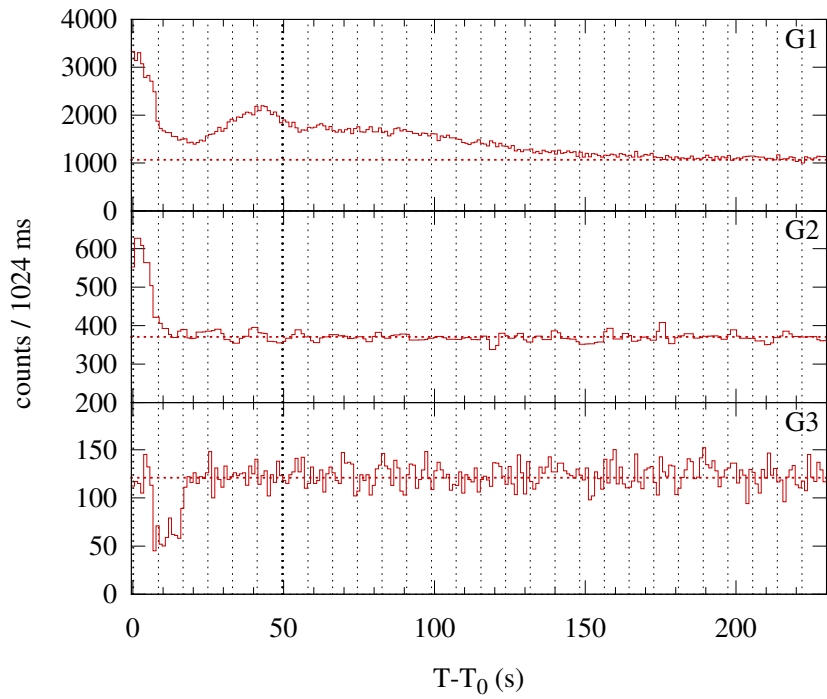
Konus-WIND S2 SOL2013-12-22T08:08 (M1.9) T_0 = 29331.393 s UT (08:08:51.393)
