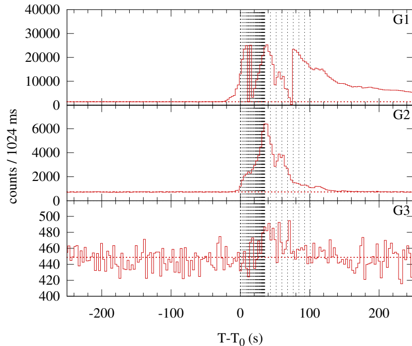
Konus-WIND S2 SOL2014-01-07T10:10 (M7.2) T_0 = 36651.201 s UT (10:10:51.201)
