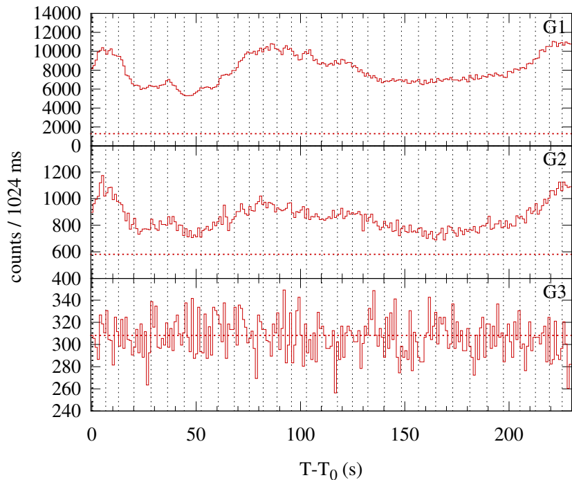
Konus-WIND S2 SOL2014-01-07T18:07 (X1.2) T_0 = 65264.794 s UT (18:07:44.794)
