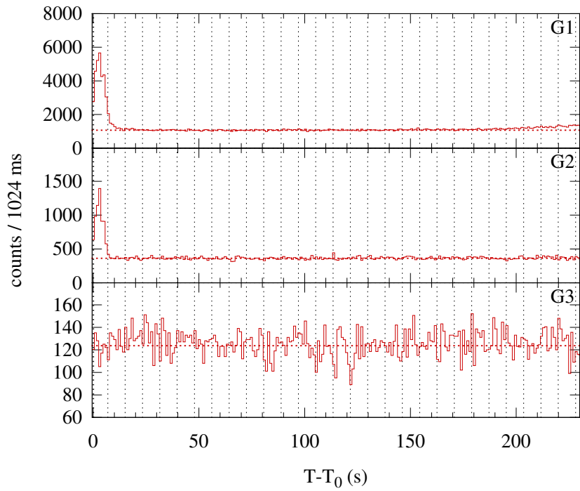
Konus-WIND S2 SOL2014-01-29T04:13 (C7.3) T 0 = 15209.995 s UT (04:13:29.995)
