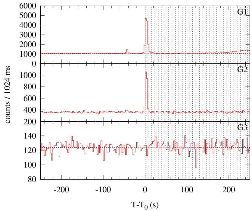
Konus-WIND S2 SOL2014-01-29T04:13 (C7.3) T 0 = 15209.995 s UT (04:13:29.995)
