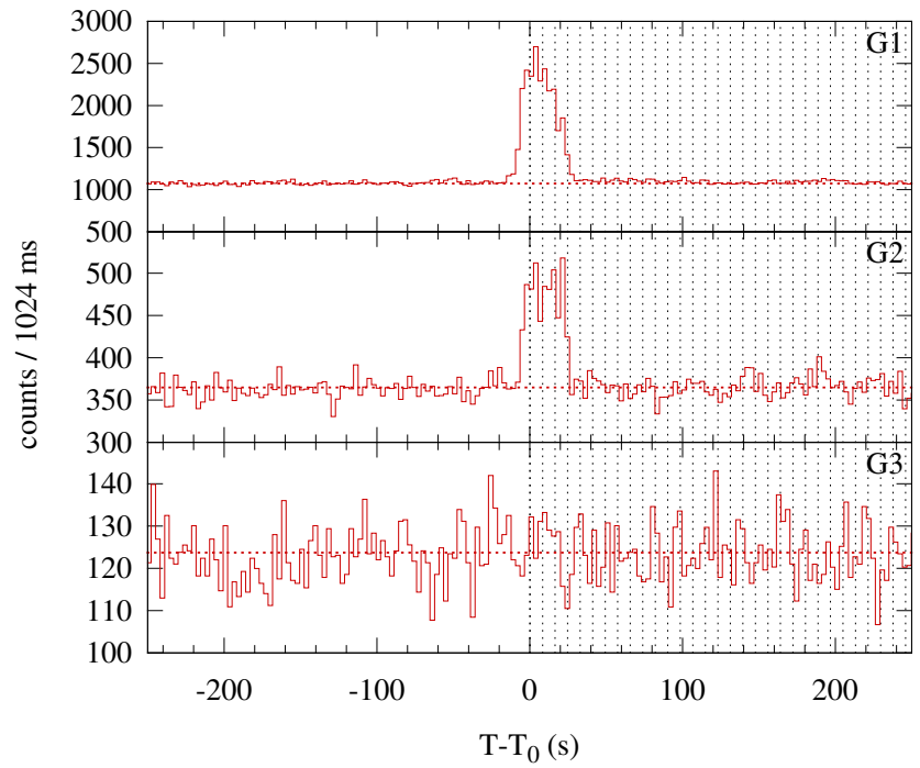
Konus-WIND S2 SOL2014-02-05T14:42 (C3.3) T 0 = 52941.404 s UT (14:42:21.404)
