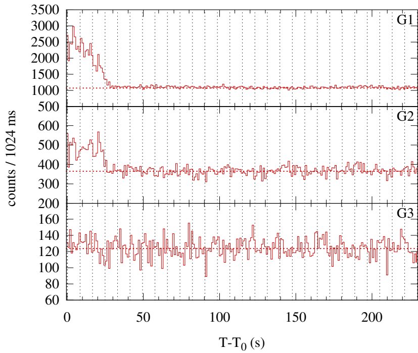
Konus-WIND S2 SOL2014-02-05T14:42 (C3.3) T 0 = 52941.404 s UT (14:42:21.404)
