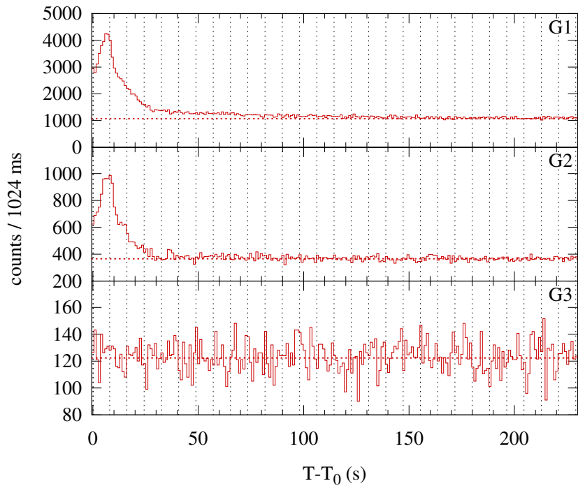
Konus-WIND S2 SOL2014-02-11T03:27 (M1.7) T 0 = 12442.944 s UT (03:27:22.944)
