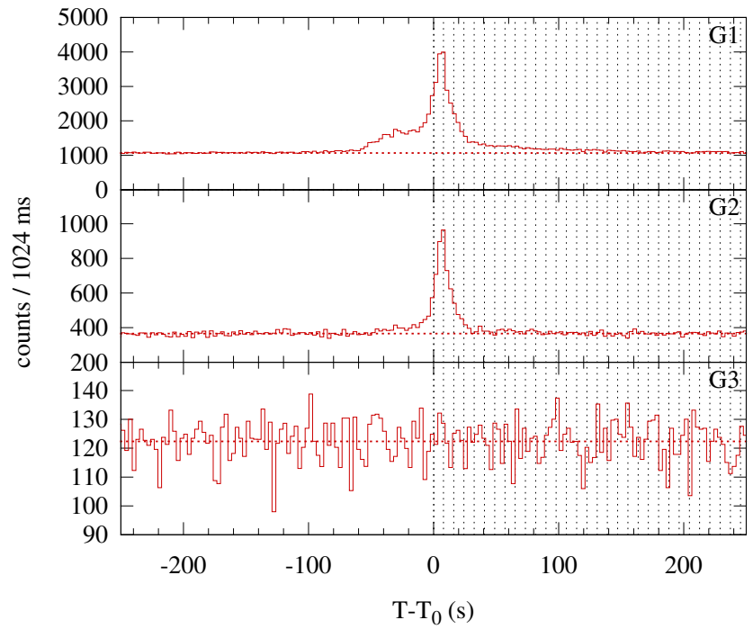
Konus-WIND S2 SOL2014-02-11T03:27 (M1.7) T 0 = 12442.944 s UT (03:27:22.944)
