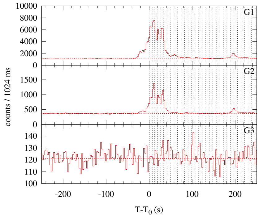
Konus-WIND S2 SOL2014-02-16T09:23 (M1.1) T_0 = 33829.594 s UT (09:23:49.594)
