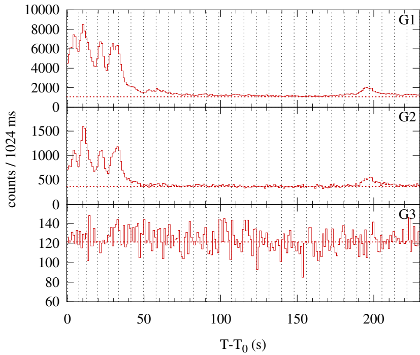
Konus-WIND S2 SOL2014-02-16T09:23 (M1.1) T_0 = 33829.594 s UT (09:23:49.594)
