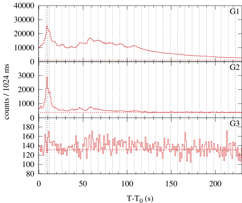
Konus-WIND S2 SOL2014-03-12T22:31 (M9.3) T_0 = 81109.228 s UT (22:31:49.228)
