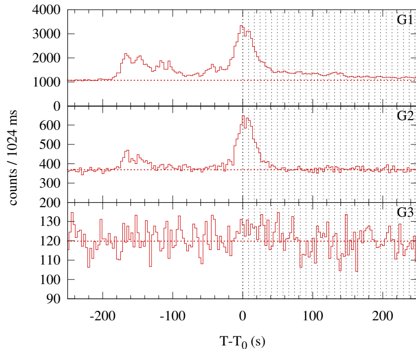
Konus-WIND S2 SOL2014-03-28T23:49 (M2.6) T_0 = 85742.910 s UT (23:49:02.910)
