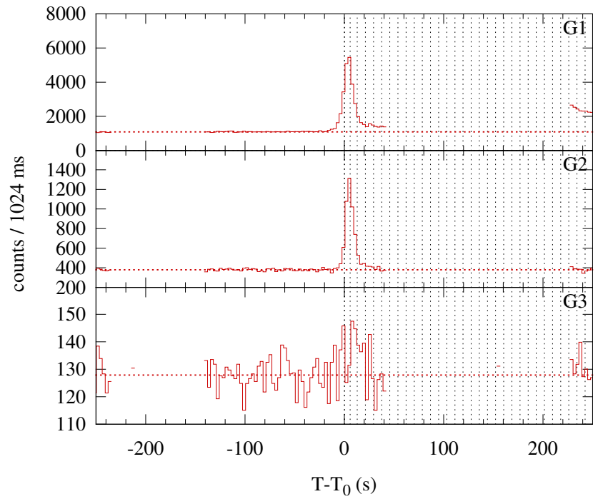
Konus-WIND S2 SOL2014-06-11T08:03 (M3.0) T 0 = 29006.838 s UT (08:03:26.838)
