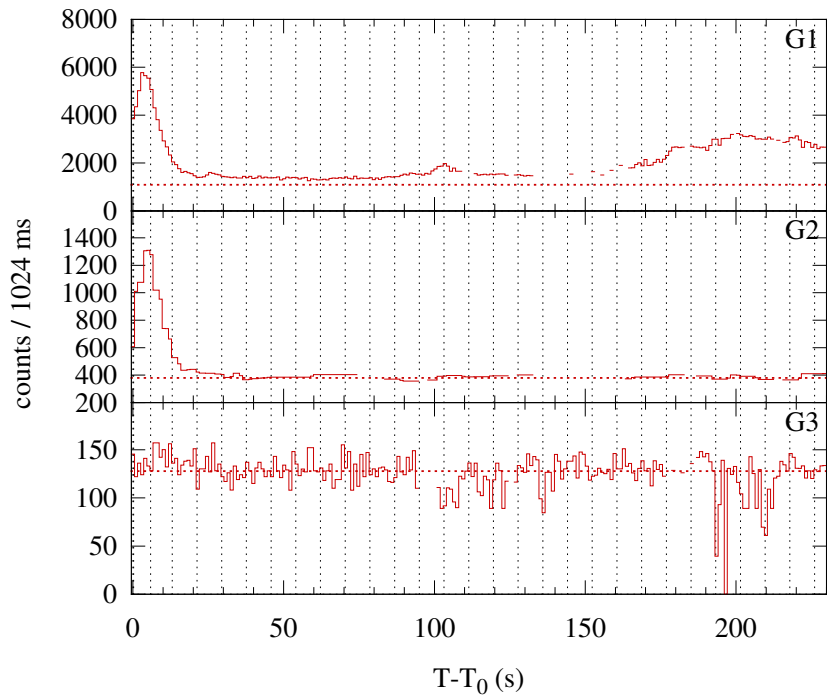
Konus-WIND S2 SOL2014-06-11T08:03 (M3.0) T 0 = 29006.838 s UT (08:03:26.838)
