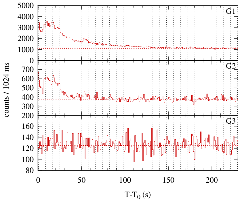
Konus-WIND S2 SOL2014-06-12T04:19 (M2.0) T_0 = 15553.10 s UT (04:19:13.10)
