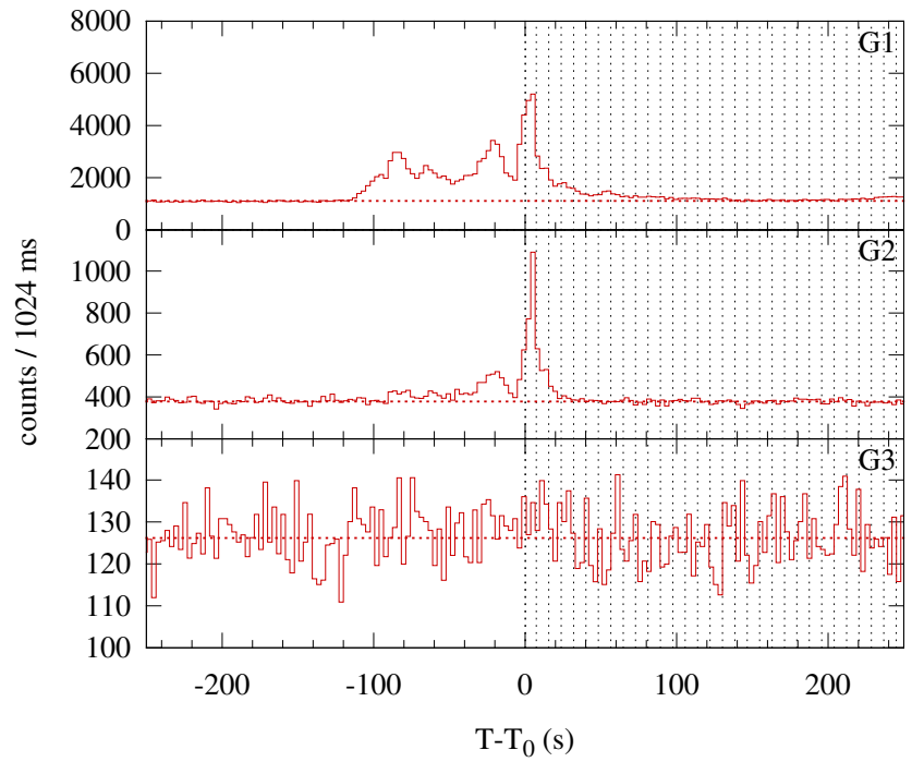
Konus-WIND S2 SOL2014-06-12T09:35 (M1.8) T_0 = 34537.886 s UT (09:35:37.886)
