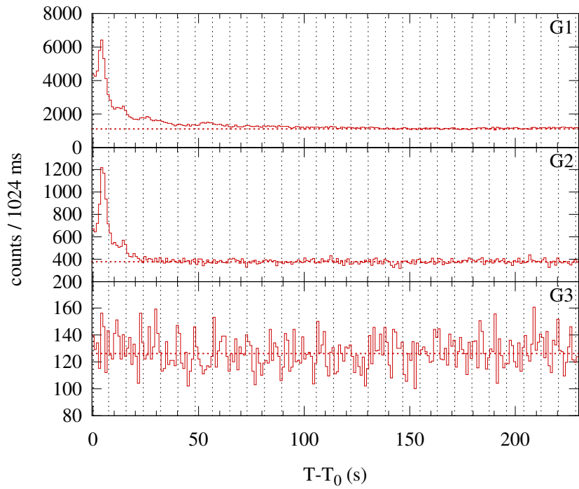
Konus-WIND S2 SOL2014-06-12T09:35 (M1.8) T_0 = 34537.886 s UT (09:35:37.886)
