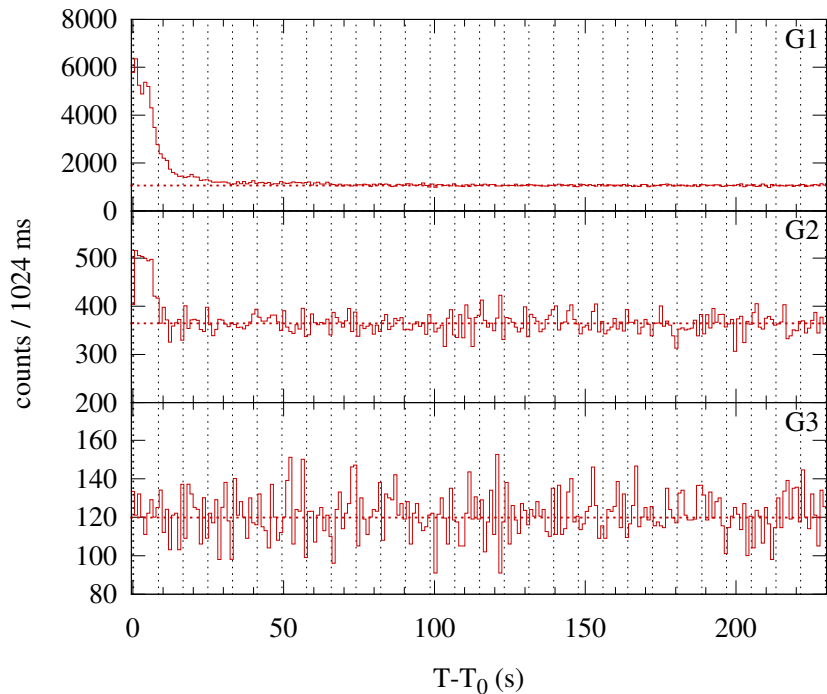
Konus-WIND S2 SOL2014-07-07T08:00 (C4.3) T_0 = 28850.814 s UT (08:00:50.814)
