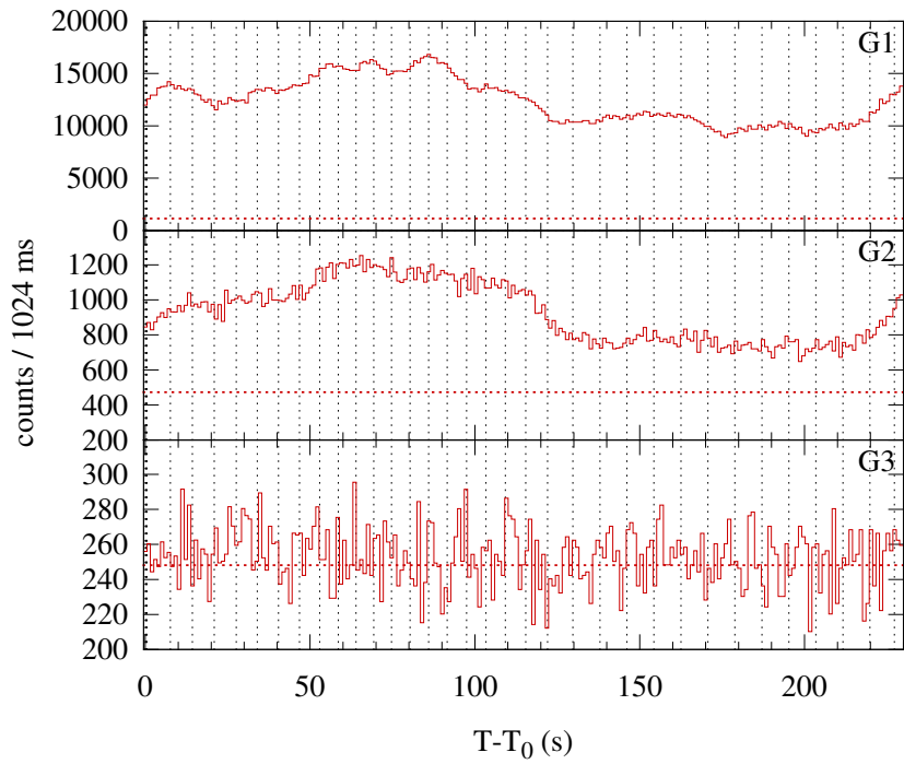
Konus-WIND S2 SOL2014-09-10T17:26 (X1.6) T_0 = 62806.13 s UT (17:26:46.13)
