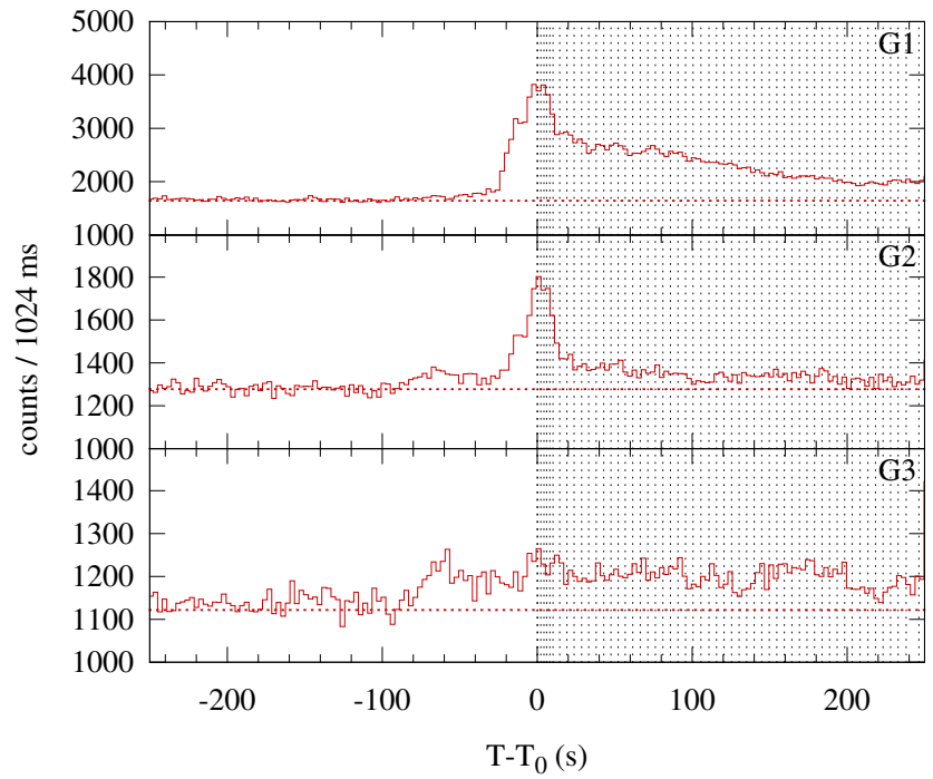
Konus-WIND S2 SOL2014-09-11T15:23 (M2.1) T 0 = 55407.962 s UT (15:23:27.962)
