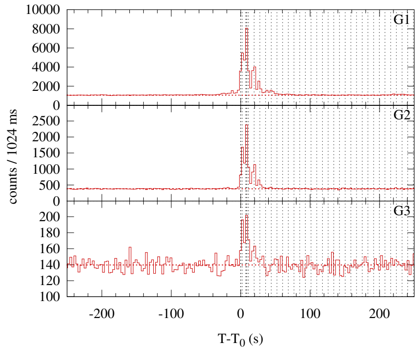
Konus-WIND S2 SOL2014-09-24T17:49 (C7.0) T 0 = 64144.729 s UT (17:49:04.729)
