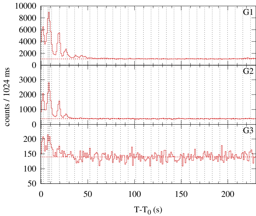
Konus-WIND S2 SOL2014-09-24T17:49 (C7.0) T 0 = 64144.729 s UT (17:49:04.729)
