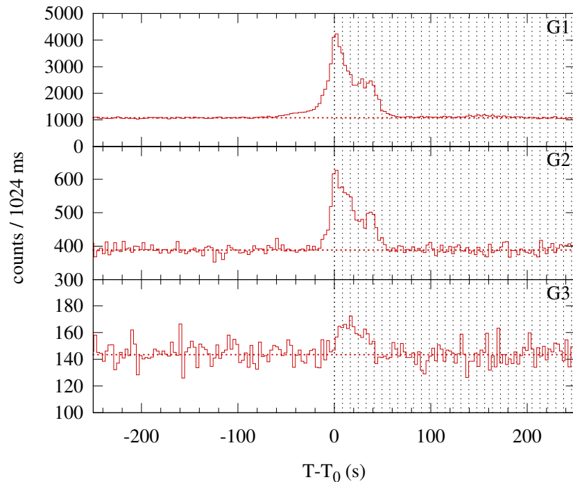
Konus-WIND S2 SOL2014-10-18T17:11 (C2.7) T_0 = 61890.163 s UT (17:11:30.163)
