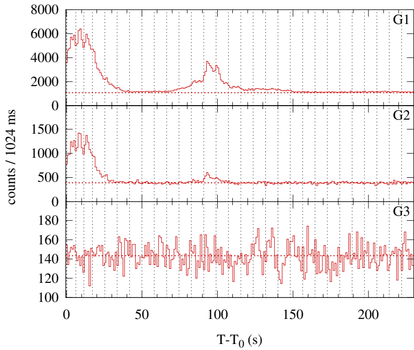
Konus-WIND S2 SOL2014-10-18T19:01 (C3.8) T_0 = 68463.604 s UT (19:01:03.604)
