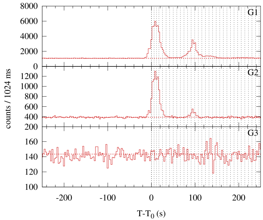
Konus-WIND S2 SOL2014-10-18T19:01 (C3.8) T_0 = 68463.604 s UT (19:01:03.604)
