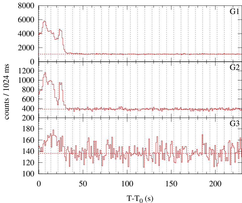
Konus-WIND S2 SOL2014-10-21T12:27 (C4.4) T 0 = 44820.465 s UT (12:27:00.465)
